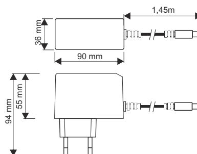
Fig.1 Dimension of power supply.
