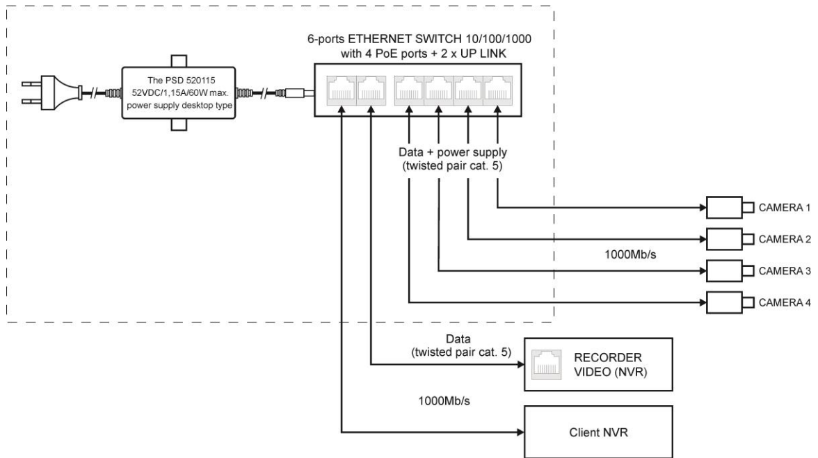
Fig. 1. Block diagram.
