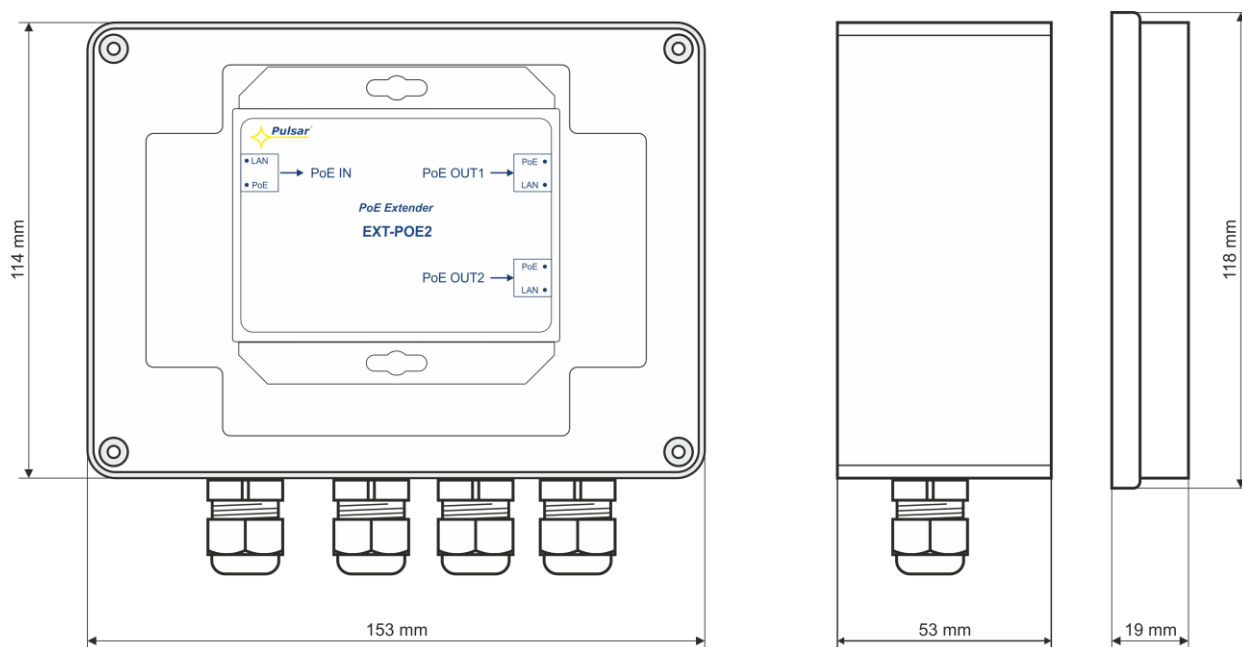
Fig. 1. View of enclosure.
