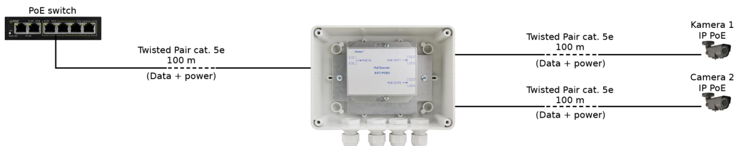
Connection of two IP PoE cameras and extension of the range for another 100m
