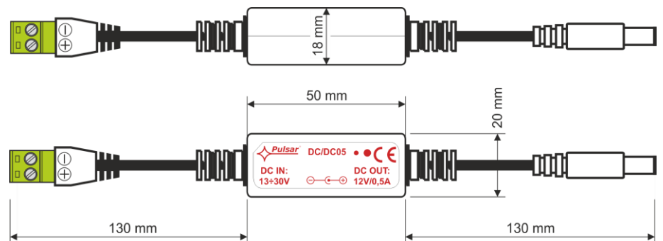
Fig.1. The mechanical diagram of the converter.
