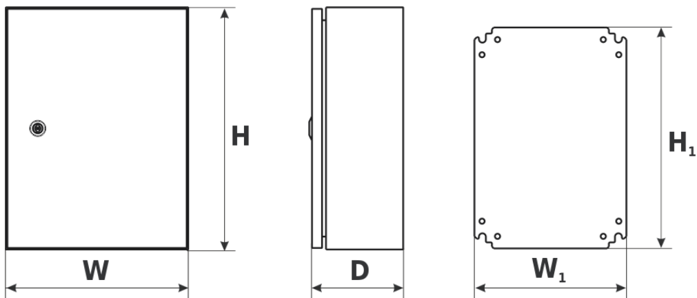
Fig. 2. Dimensions.
